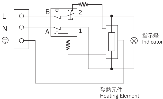
溫度調節/超溫斷路器 Combined Thermostat/Cut-Out
